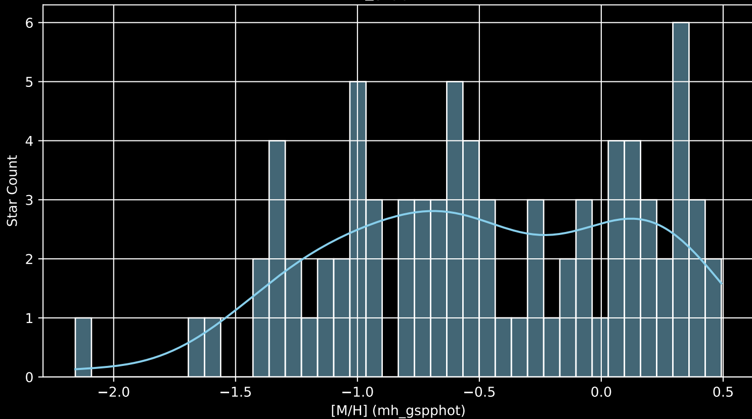
APOGEE DR17 Field: [350+00 [M/H] (mh_gspphot) (n= 81)
