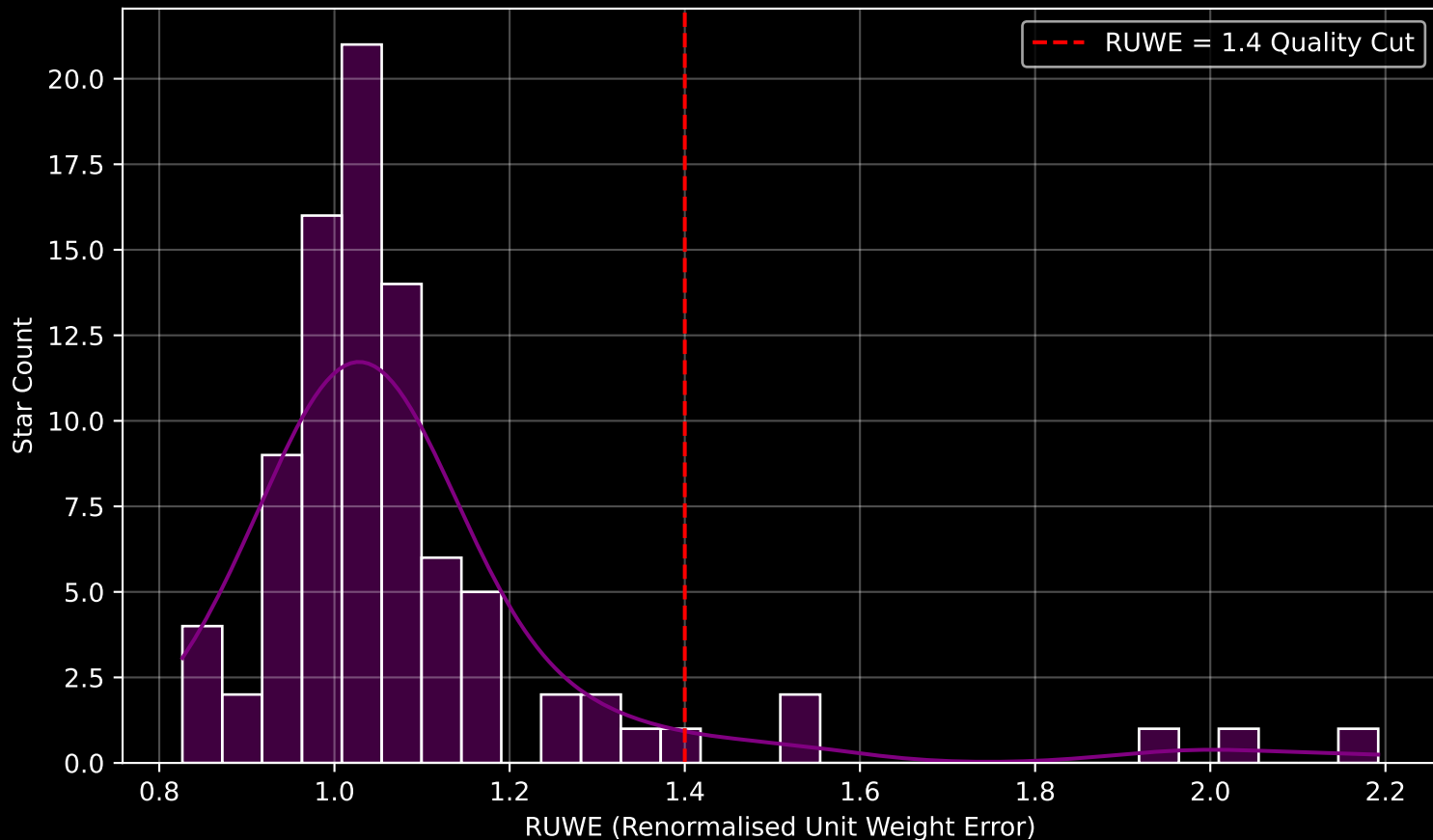
GAPOGEE DR17 Field [350+00] RUWE Distribution (n= 88)
