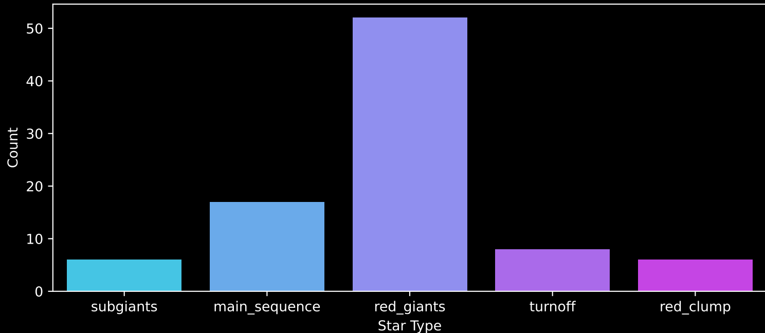
APOGEE DR17 Field: [350+00] Count plot of Star Type
