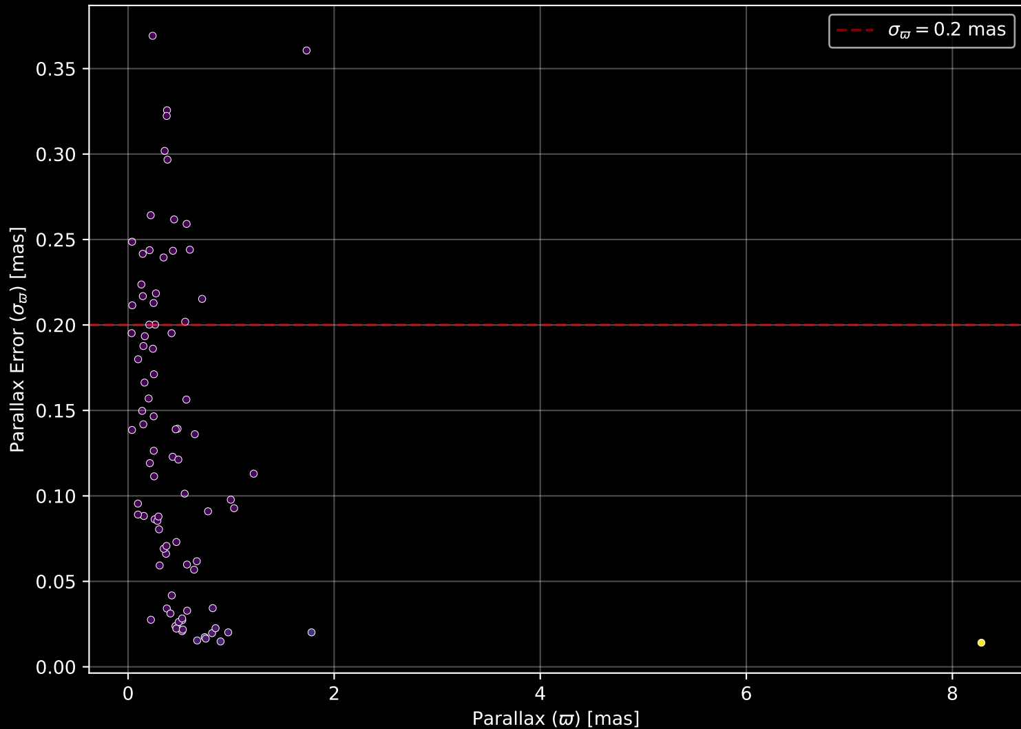
APOGEE DR17 Field: [350+00] Parallax Quality (n= 89)
