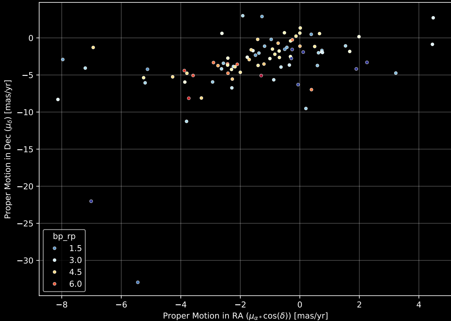
APOGEE DR17 Field: [350+00] Proper Motion Diagram (n= 89)
